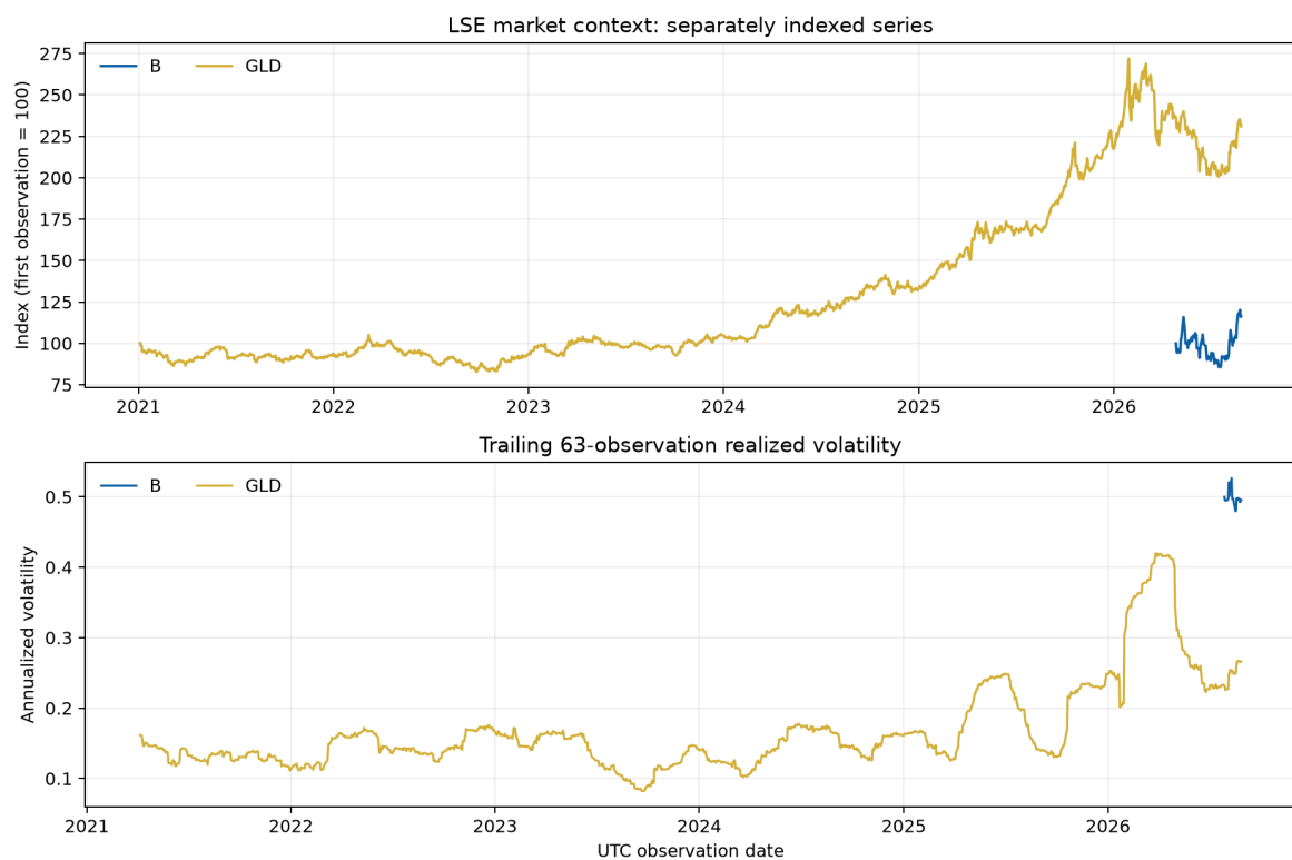
Figure 3.1: Separately indexed LSE series and trailing 63-observation realized volatility. Barrick B is shown only over the catalog-valid interval; GLD is an ETF proxy in USD/share. The discontinuous coverage is deliberate and prevents an unsupported GOLD→B stitch.
