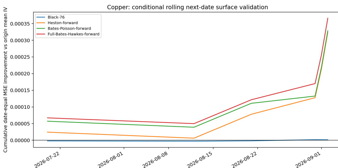
Figure 10.5: Cumulative date-equal MSE improvement against origin-mean IV. Only actual admitted targets enter; elapsed gaps are preserved. Positive improvement against this benchmark need not imply improvement against surface persistence.
