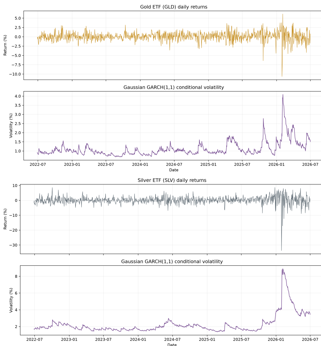
Figure 7.8: Current LSE Gaussian GARCH(1,1) conditional volatility for GLD and SLV
